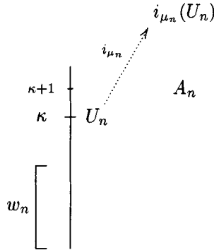
Diagram 4. Pushing U_n up.
