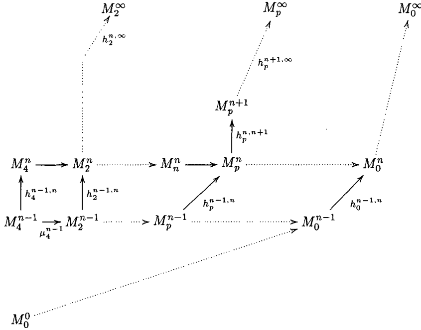
Diagram 6. The direct limits M_k^\infty .
