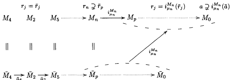
Diagram 5. \{M_j, \mu_j, r_j, a\} extends \{\bar{M}_j, \bar{\mu}_j, \bar{r}_j, \bar{a}\} .
