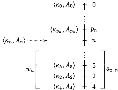
Diagram 2. Configuration at round n of the repeated rank game.
